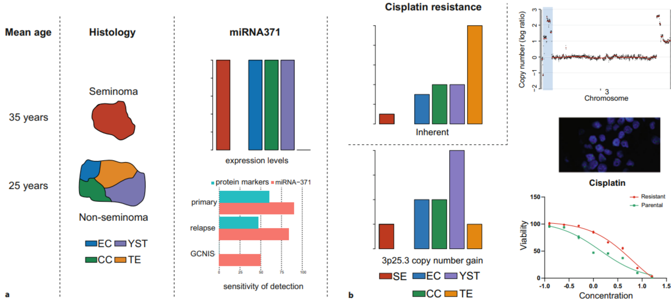
Fig. 1 Schematic representation of the histological subtypes in type II germ cell tumors and their characteristics regarding miRNA-371 expression (a) and their cisplatin resistance (b)
